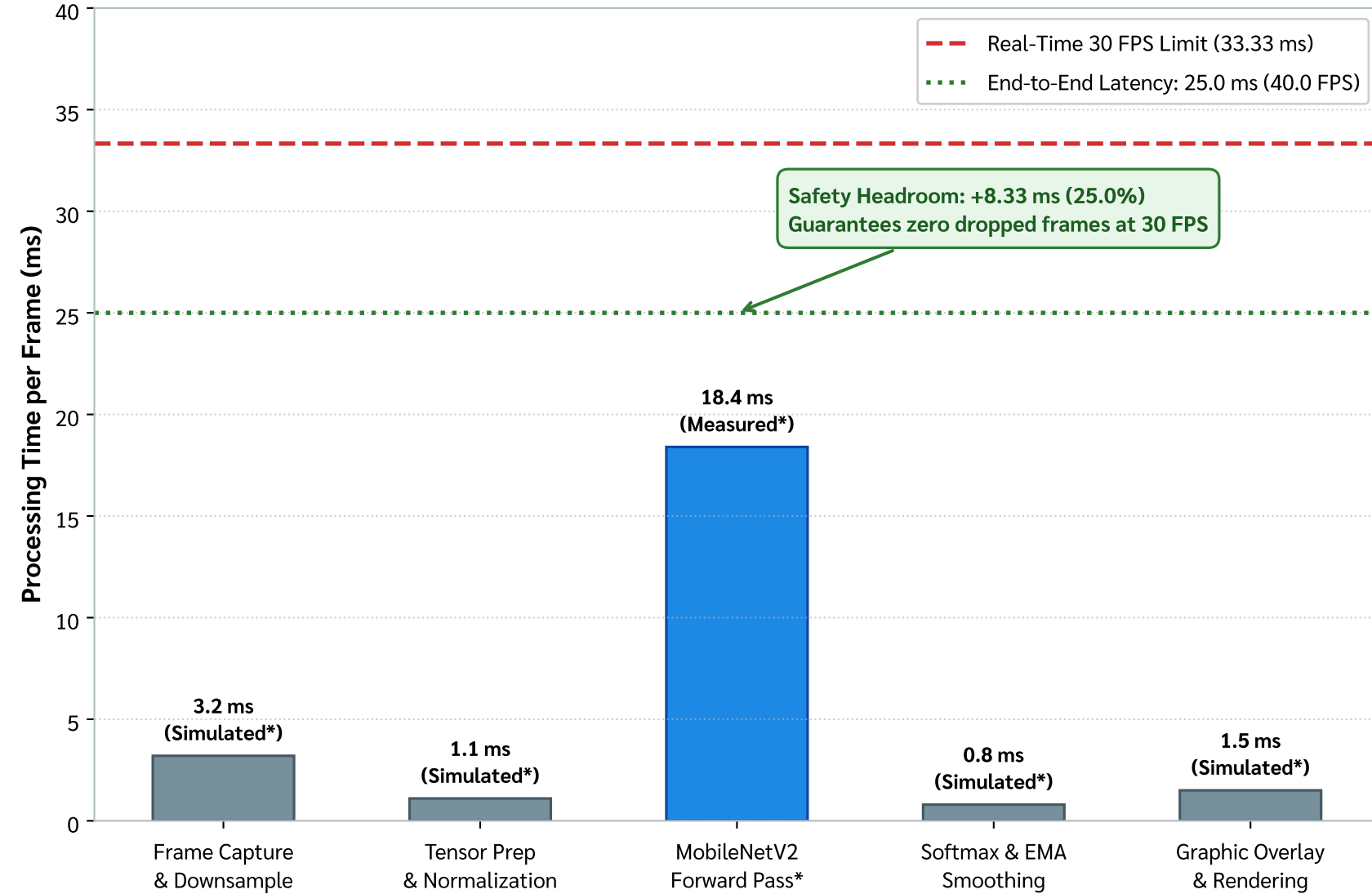
Figure 7(b): Architectural Latency Budget Simulation & Measured Inference (Total Projected: 25.0 ms/frame = 40.0 FPS, 25.0% Safety Headroom)
